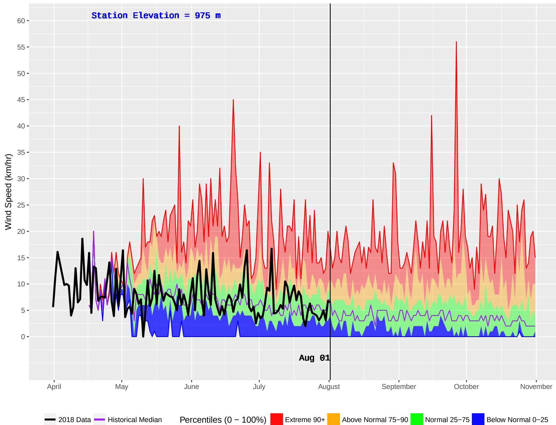
MCGREGOR 2 (192) : Historical (1986–2016) and Current (2018) Daily Wind Speed
